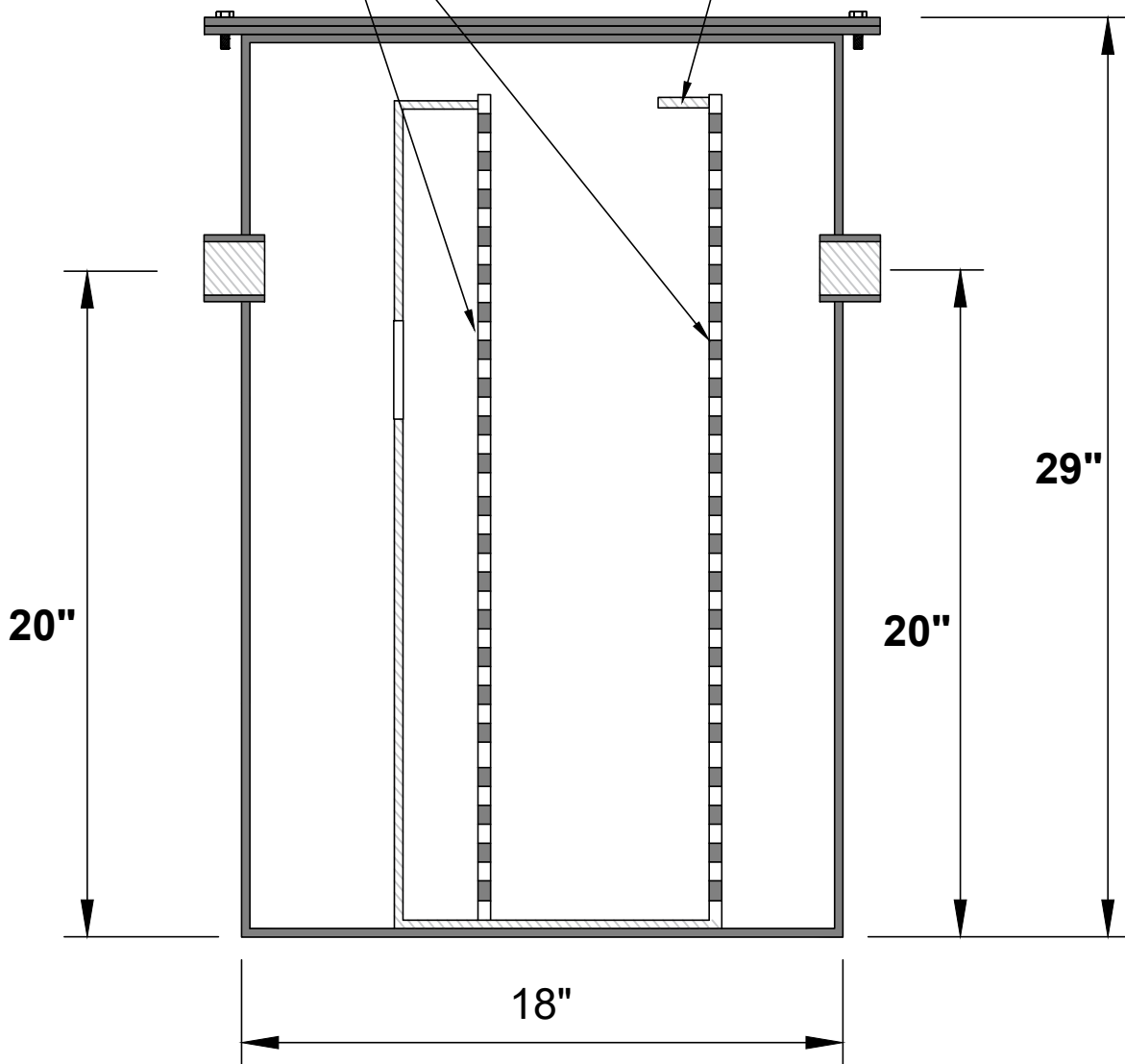
SECTION VIEW
