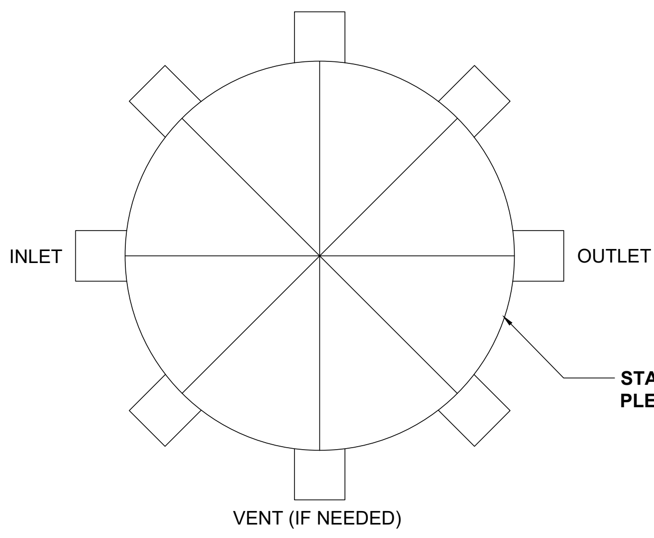
TOP VIEW
