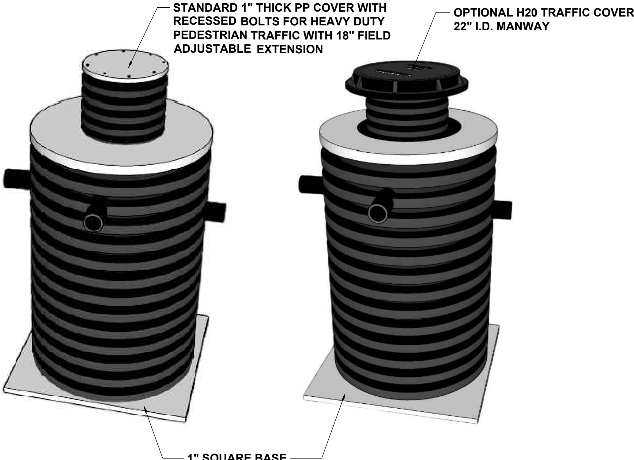
1" SQUARE BASE
