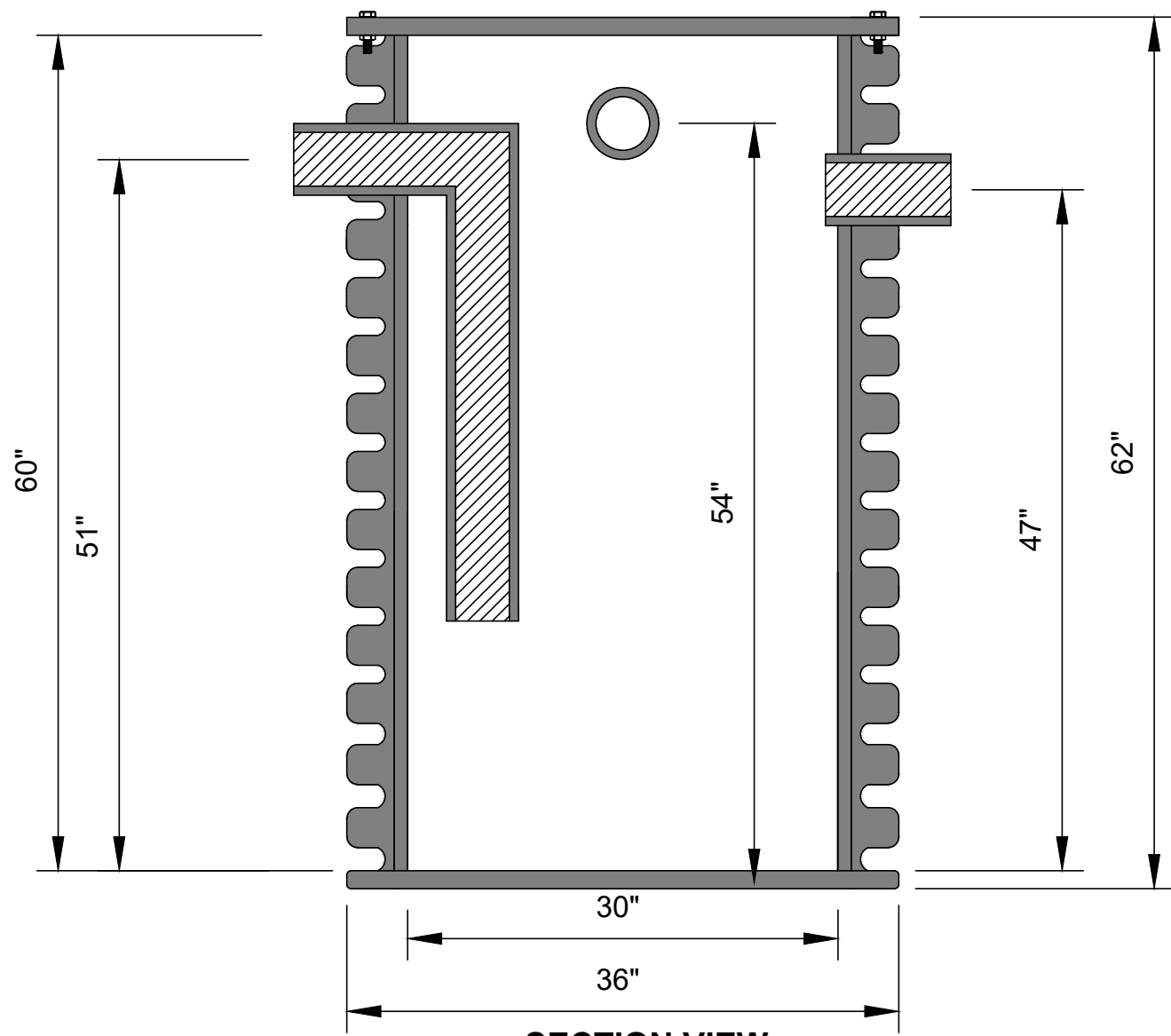
SECTION VIEW
