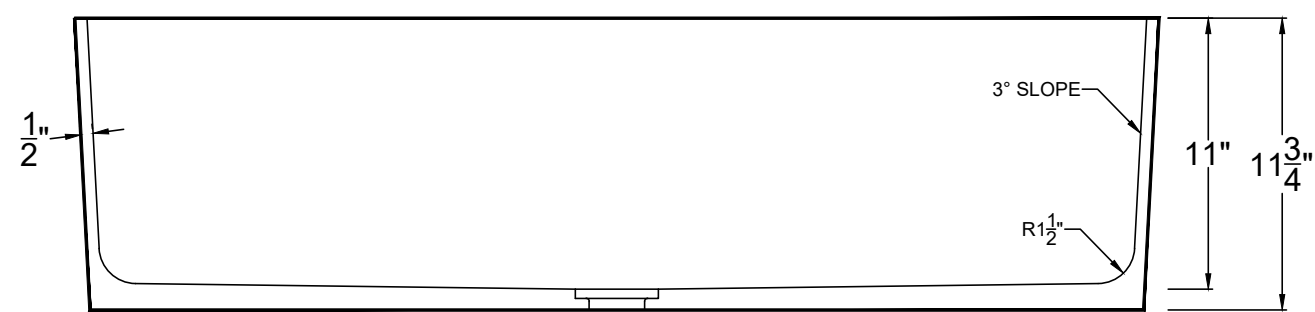
SECTION VIEW
