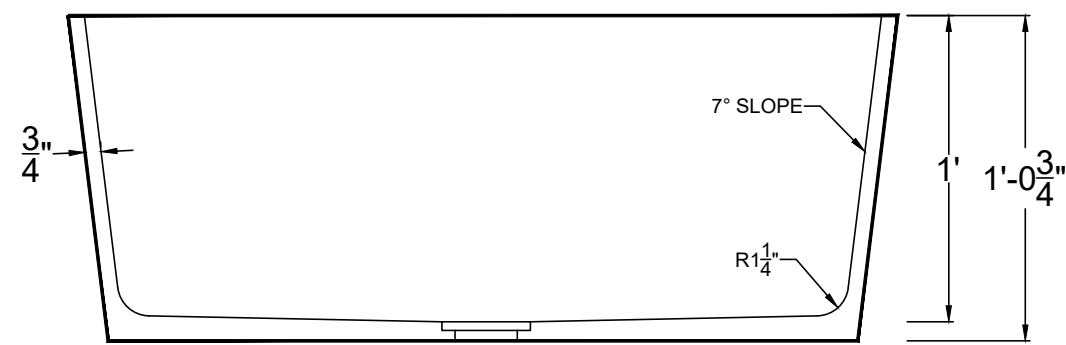
SECTION VIEW
