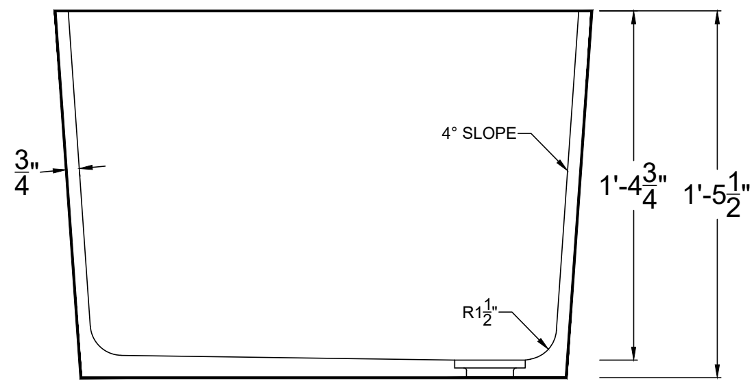
SECTION VIEW
