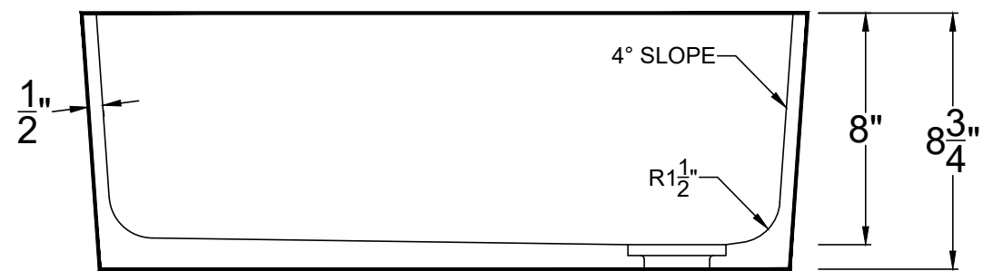
SECTION VIEW
