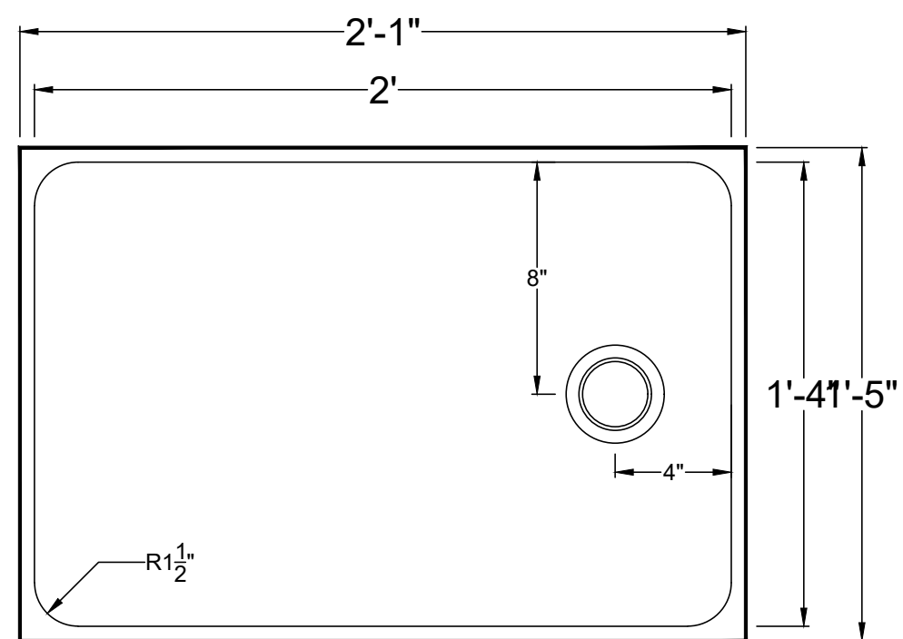
TOP VIEW
