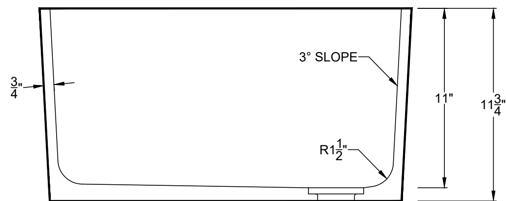
SECTION VIEW
