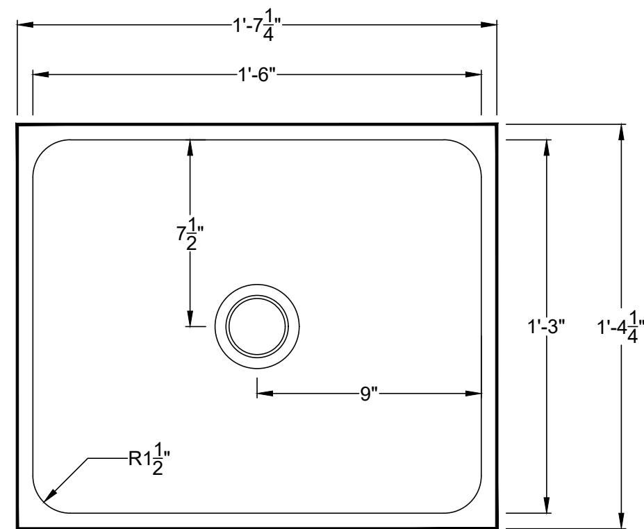
TOP VIEW
