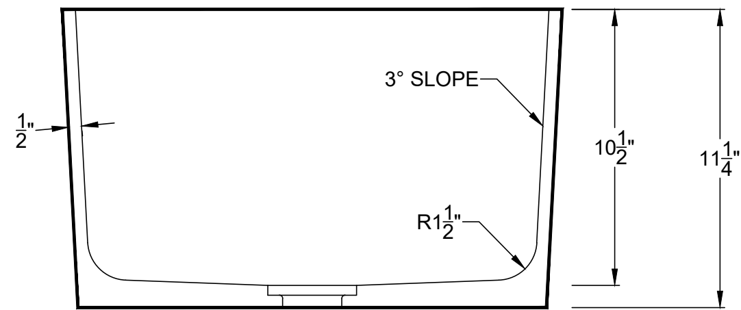
SECTION VIEW
