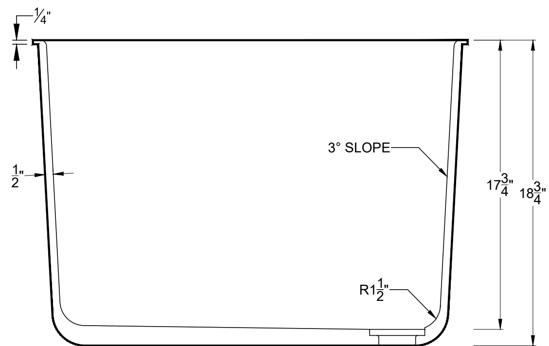
SECTION VIEW
