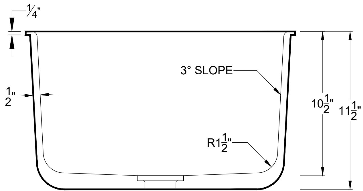
SECTION VIEW
