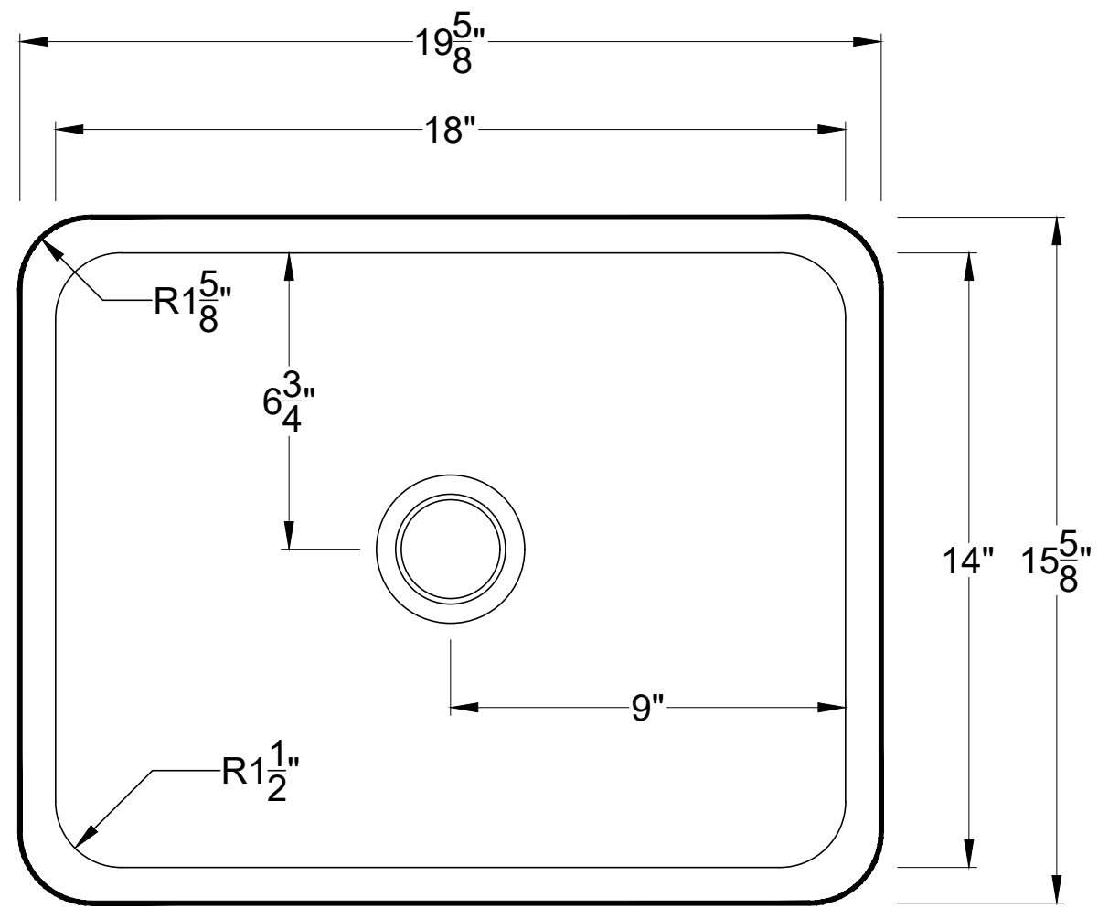
TOP VIEW
