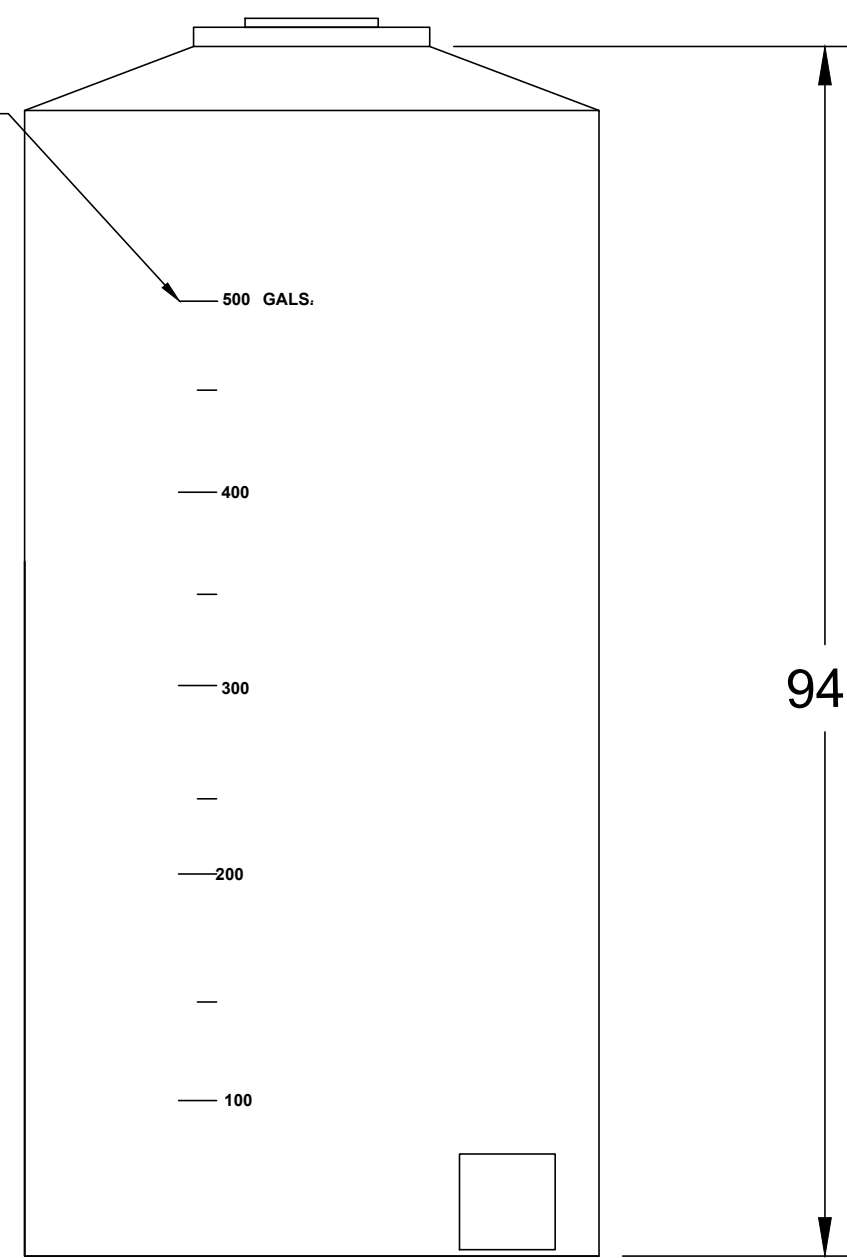
SECTION VIEW
