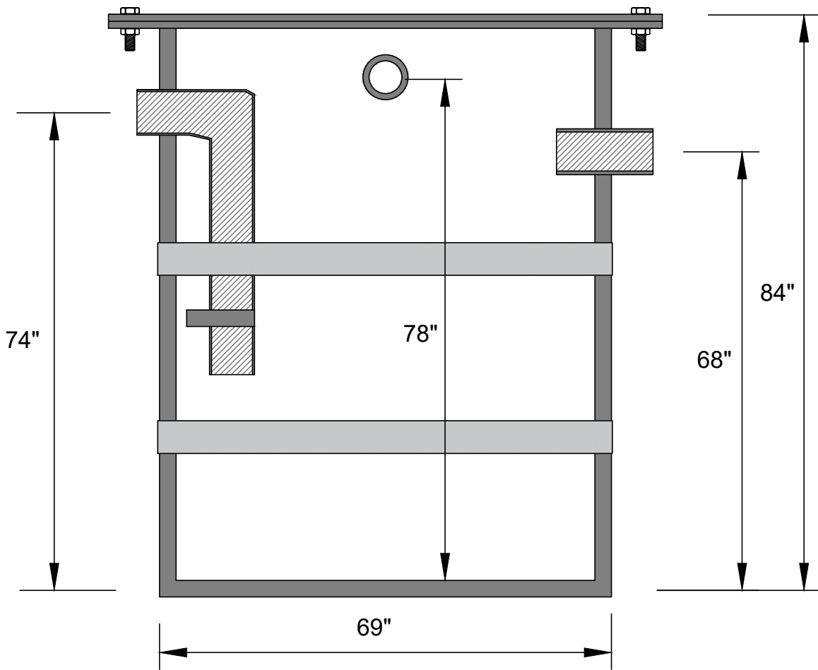
SECTION VIEW
