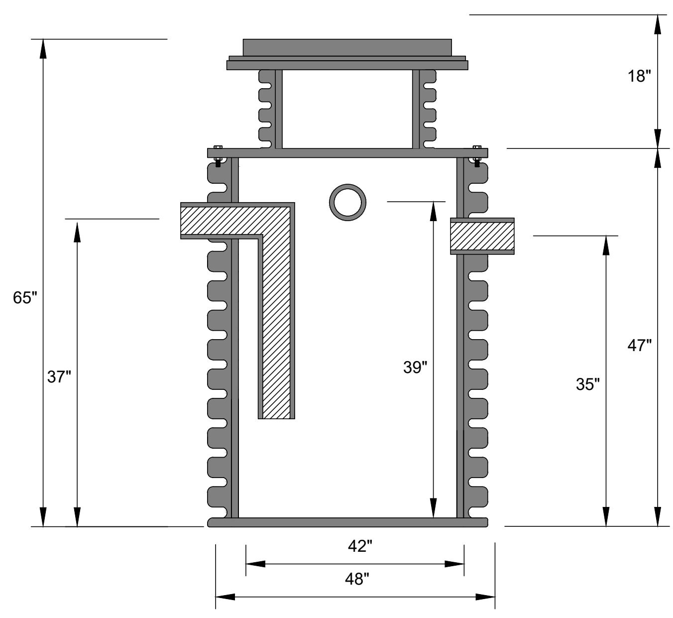
SECTION VIEW
