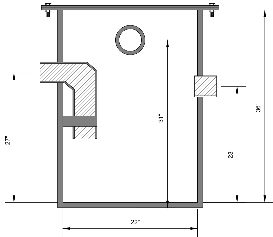
SECTION VIEW
