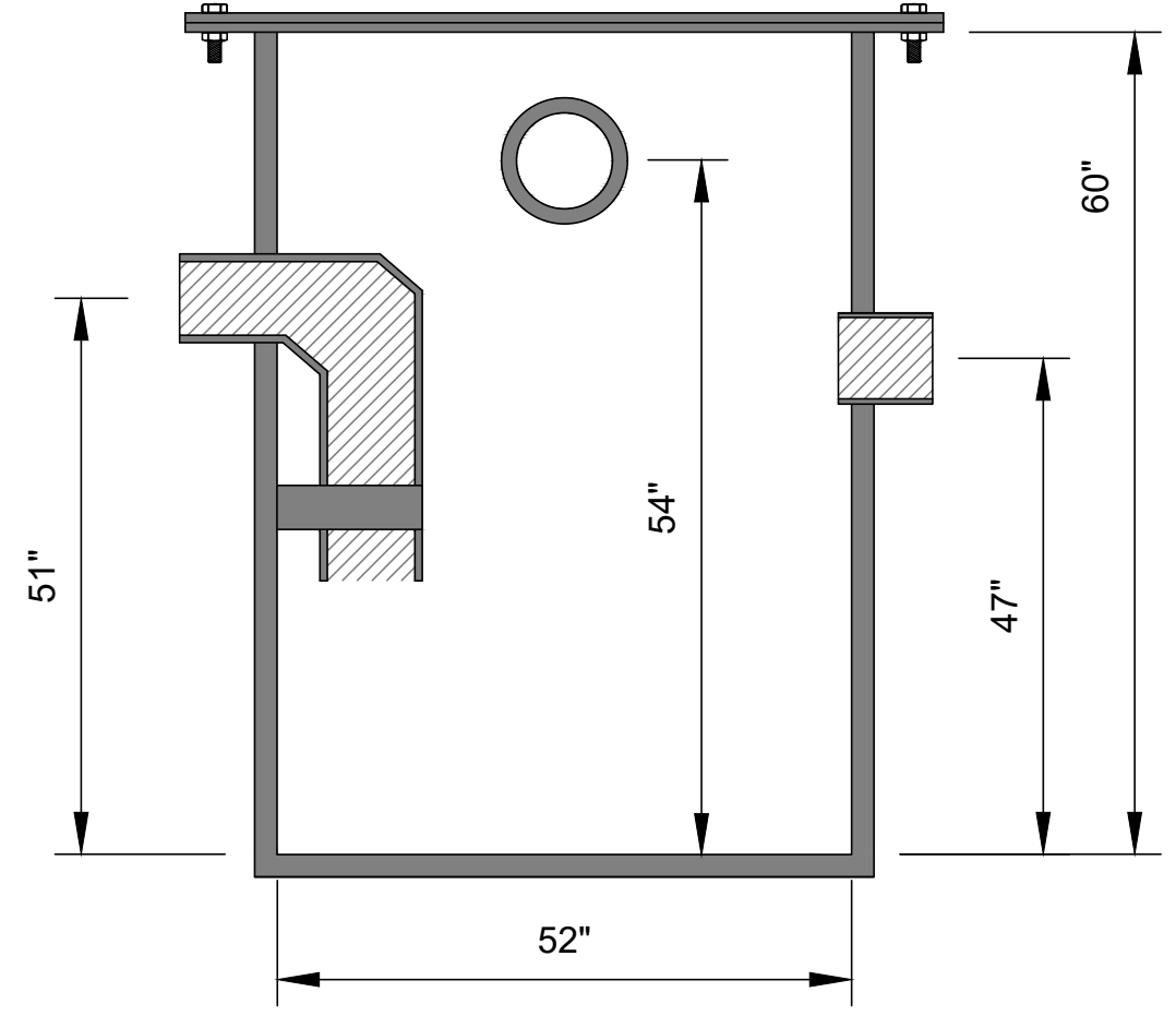
SECTION VIEW
