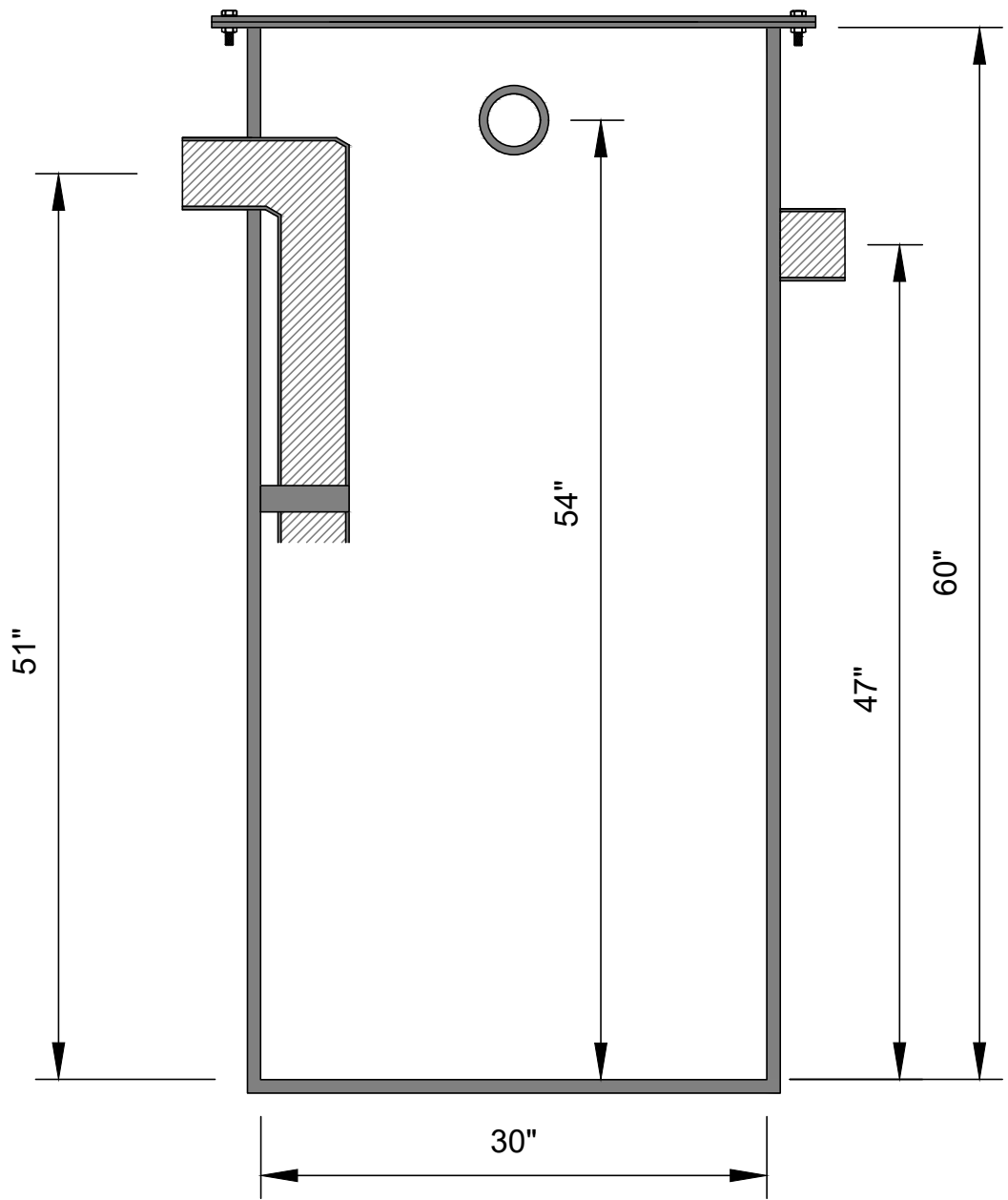
SECTION VIEW
